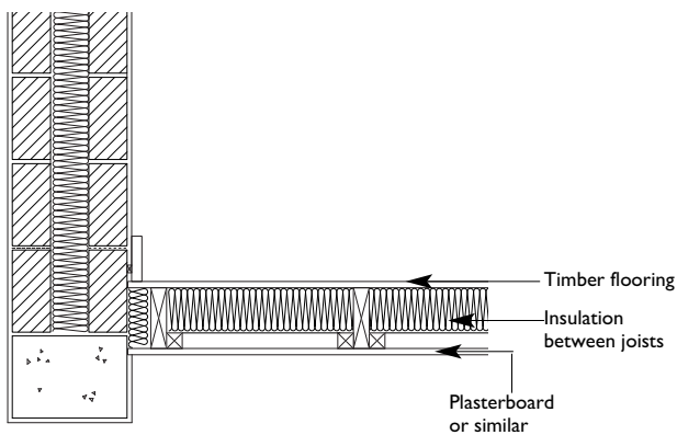
Diagram B21 Para. B.7.4 Exposed timber floor, insulation between joists
